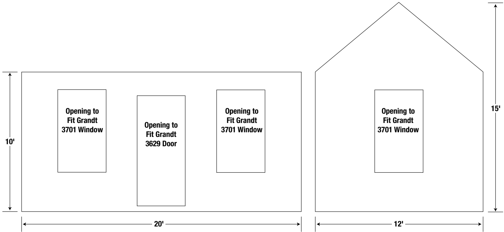
Winnecook Flapstop Cutting Diagram. Sides and Ends are Identical (no Door Opening on rear of Flagstop).
