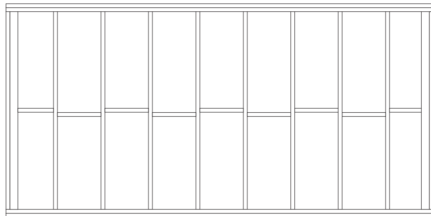
Speeder Shed Framing – O Scale By Bob Boudreau ©2011 Carstens Publications, Inc.
